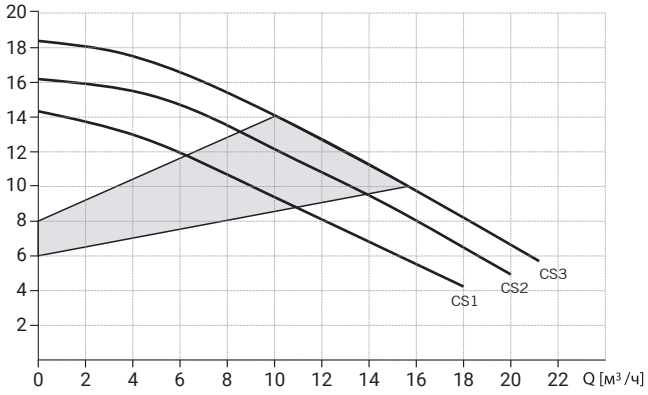
WRE BASIC 40-180F (220V)
