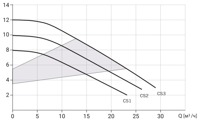
WRE BASIC 50-120F (220V)
