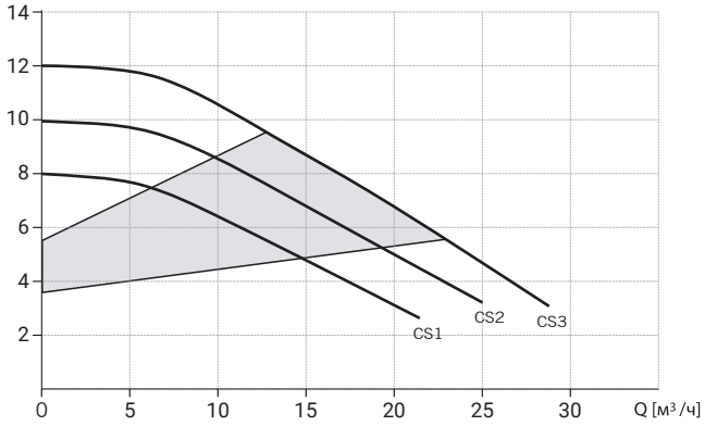
WRE BASIC 50-120F (380V)
