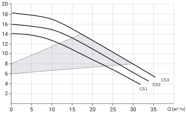
WRE BASIC 50-180F (380V)
