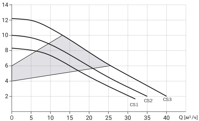
WRE BASIC 65-120F (380V)
